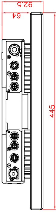
bottom view
