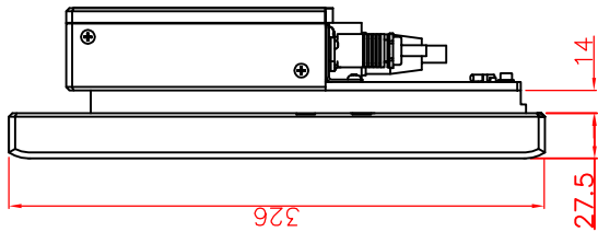
right view
