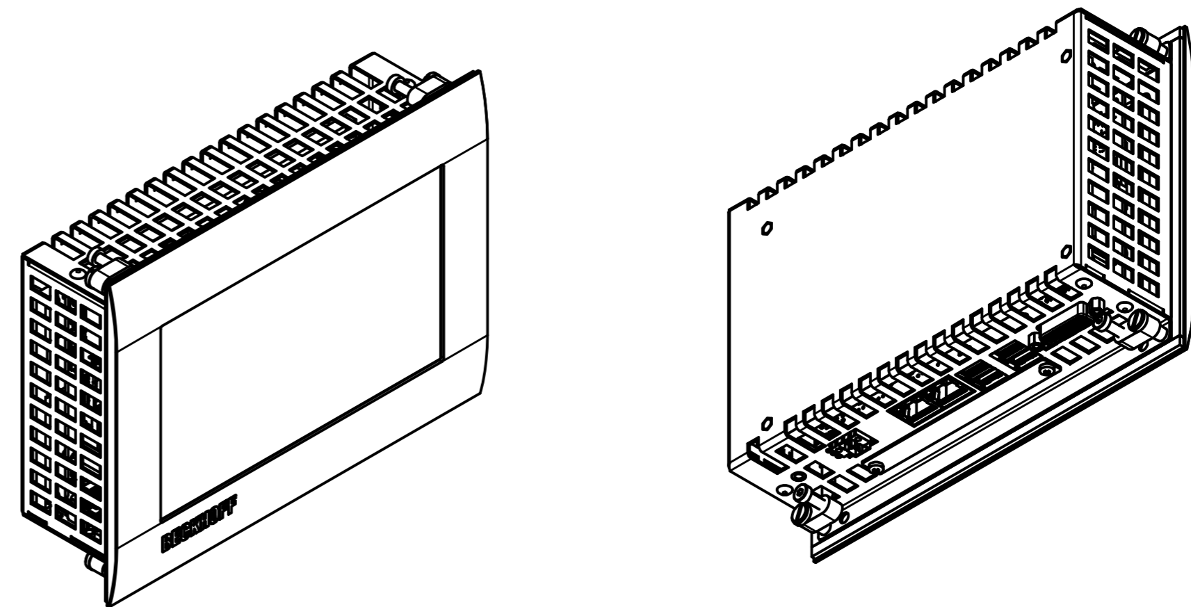
CP6706-0001 main dimensions
