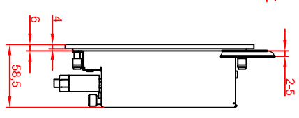
right view
