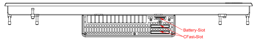
top view
