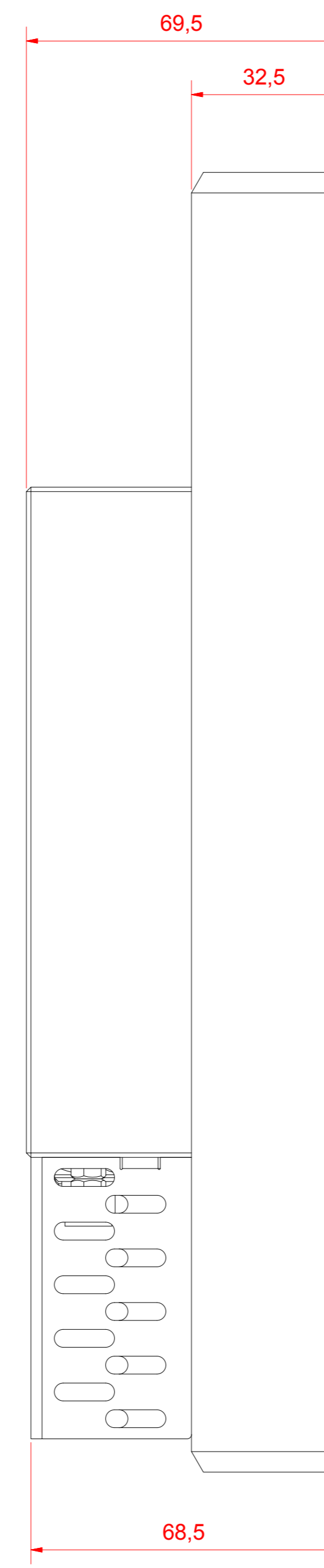
left view
