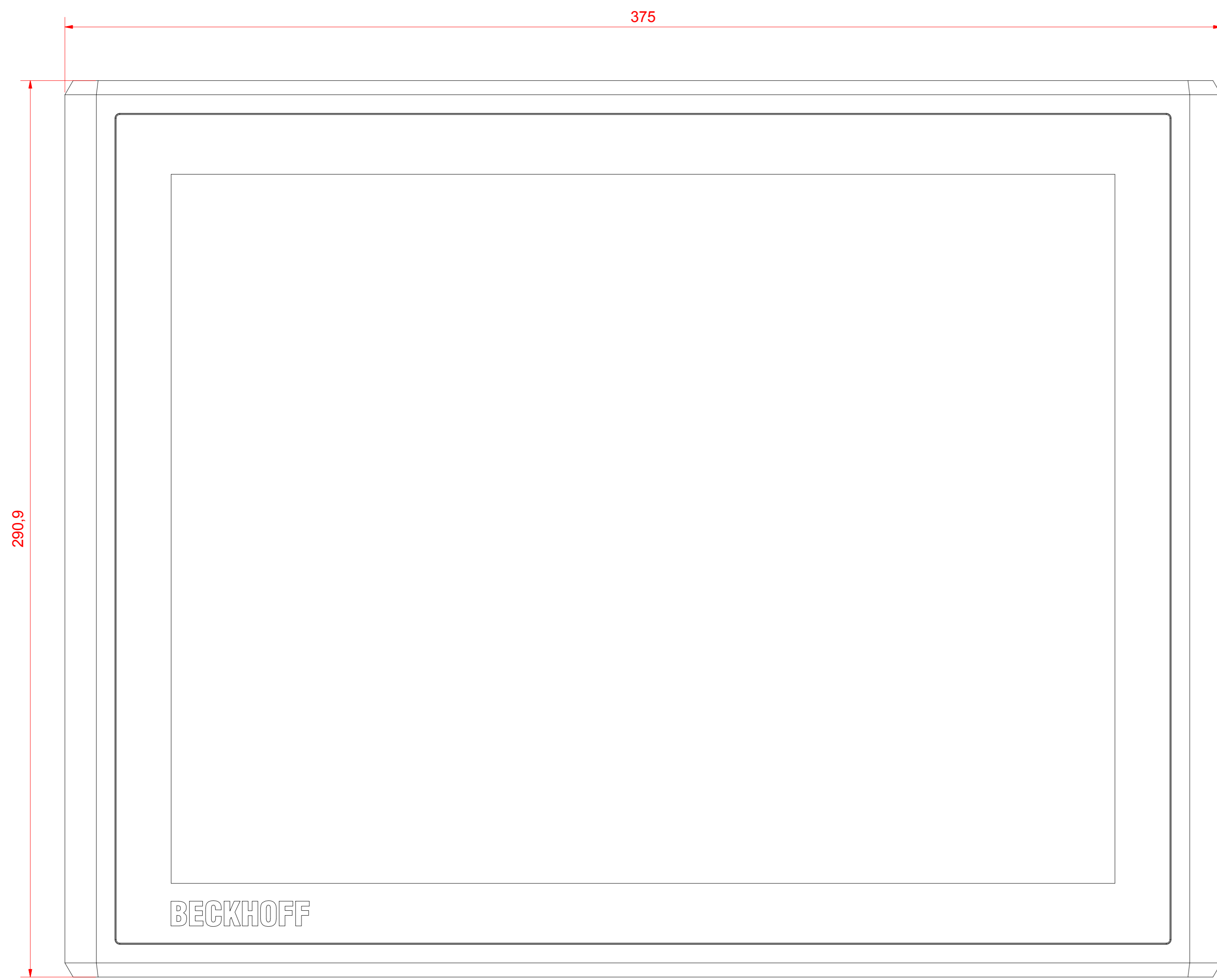
front view
