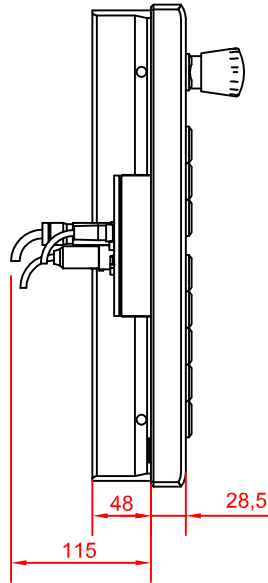
left view
