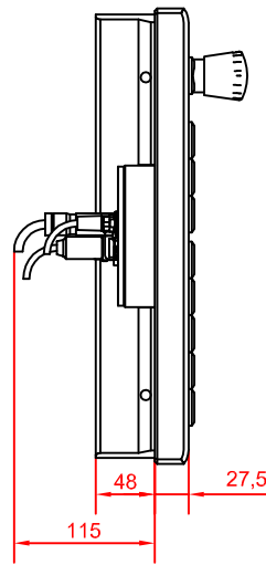
left view
