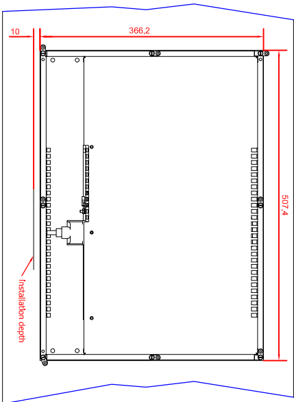
rear view with install measure
