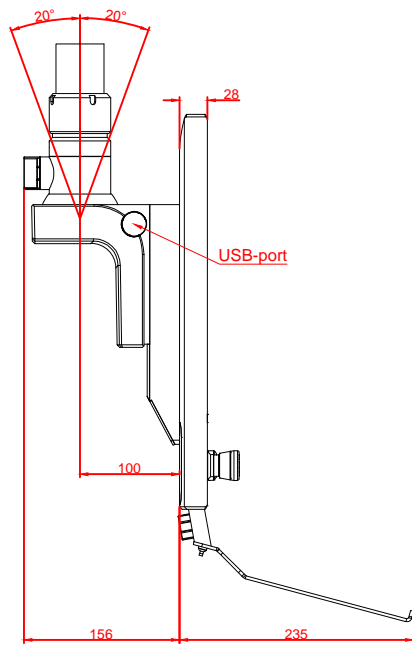
left view
