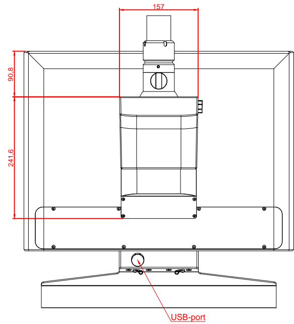
rear view
