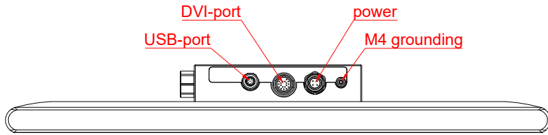
bottom view
