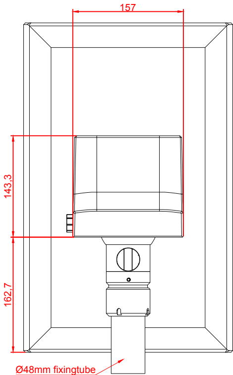
rear view
