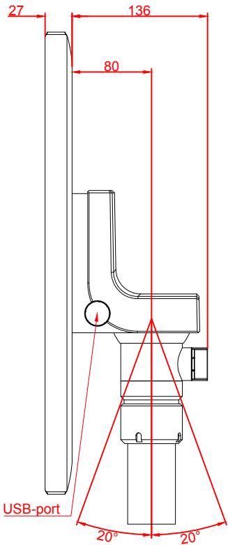
right view
