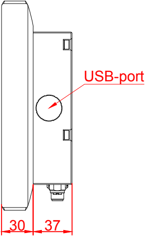
left view
