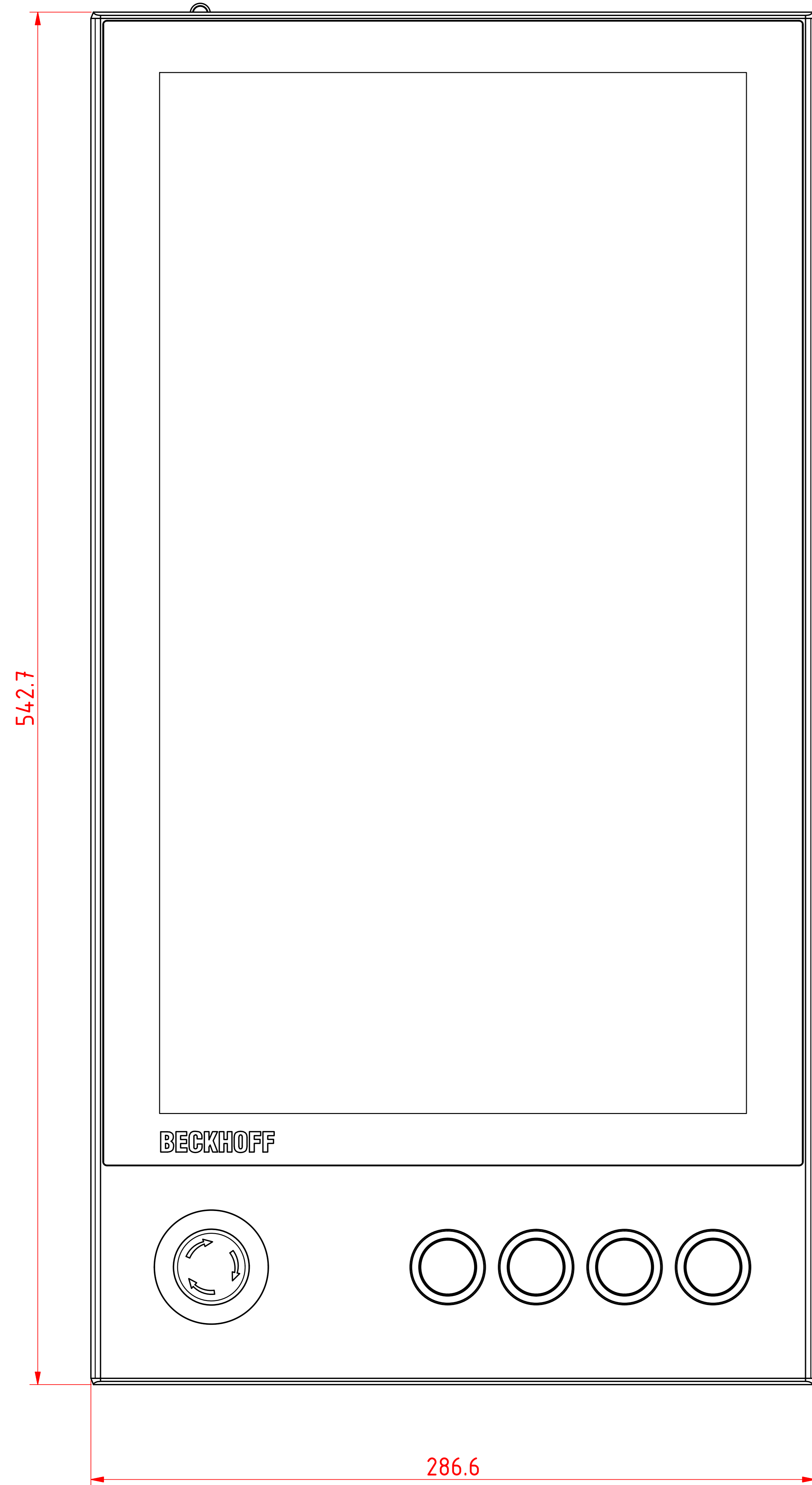
front view
