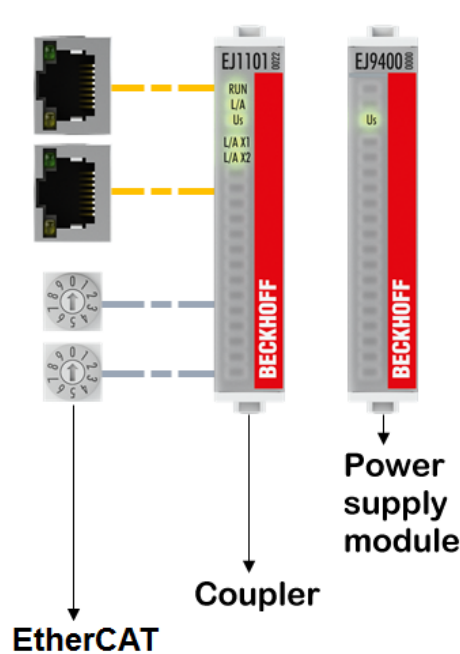
Fig. 14: E-bus power supply with EJ1100 or EJ1101-0022 + EJ940x
