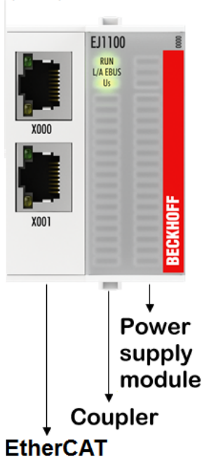
Fig. 14: E-bus power supply with EJ1100 or EJ1101-0022 + EJ940x
