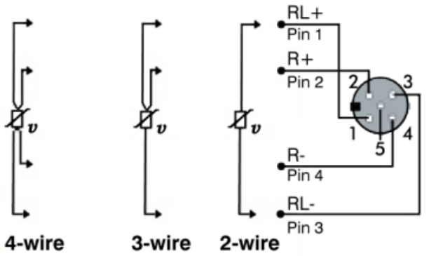
Fig. 12: Resistance measurement with a 4-wire, 3-wire and 2-wire connection technique
