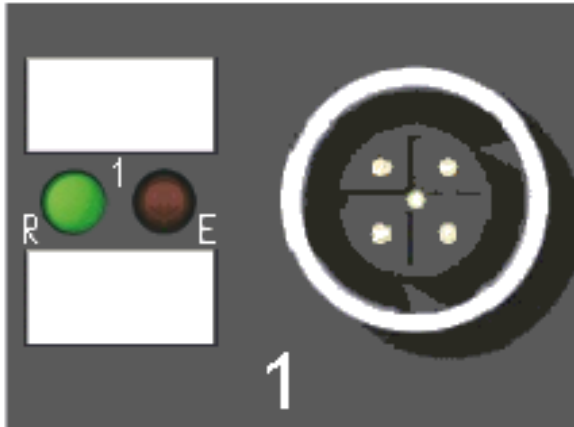
Fig. 5: Status LEDs at the signal connections
