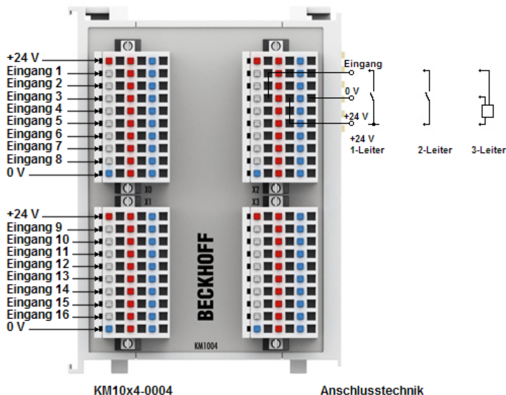
Abb. 9: KM10x4-0004
