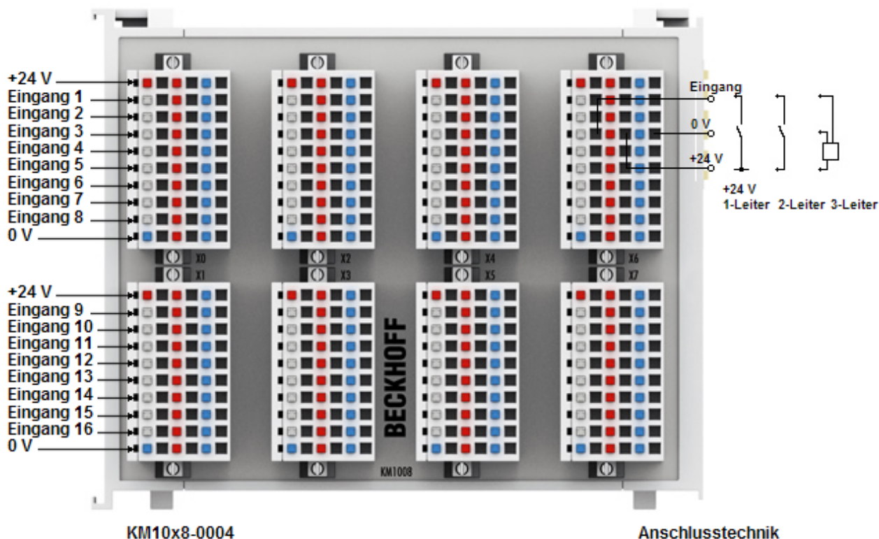
Abb. 10: KM10x8-0004
