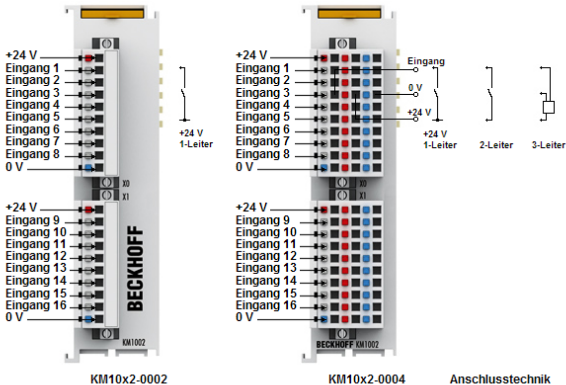
Abb. 8: KM10x2-0002, KM10x2-0004
