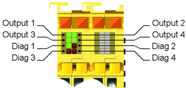
Abb. 14: Diagnose LEDs
