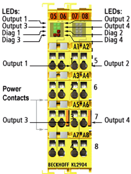
Abb. 4: KL2904
